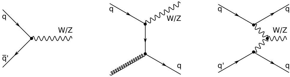
Figure 4.2: Example Feynman diagrams of W and Z boson production at hadron colliders. The subsequent decays of the produced bosons are not shown. The process shown on the right is suppressed with respect to the other processes because it involves multiple electroweak couplings.
