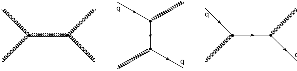
Figure 4.4: Example Feynman diagrams of the QCD multijet background.
