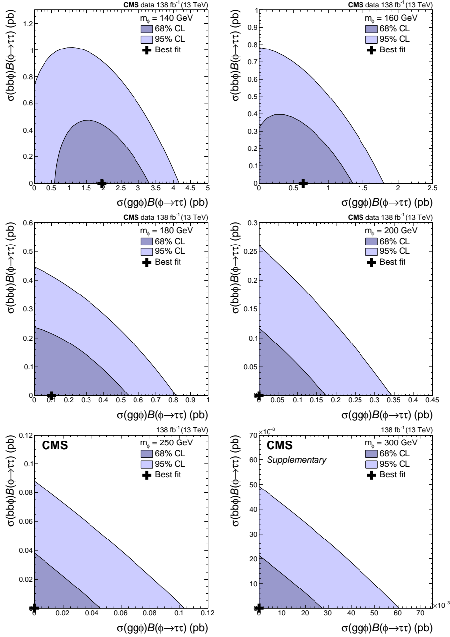
Figure B.7: Scans of the profile likelihood function in terms of \sigma_{\text{gg}\phi}\mathcal{B}(\phi \rightarrow \tau\tau) and \sigma_{\text{bb}\phi}\mathcal{B}(\phi \rightarrow \tau\tau) . The 68 and 95% CL contours are shown in dark and light purple, respectively. The best fit points are indicated by black crosses. The contours are shown for m_\phi = 140, 160, 180, 200, 250, and 300 GeV from left to right and top to bottom. Lower row published in [30].
