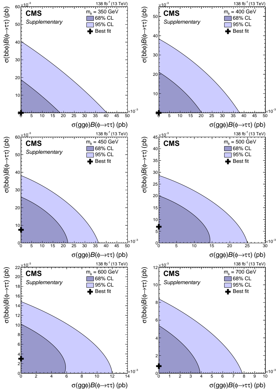
Figure B.8: Scans of the profile likelihood function in terms of \sigma_{gg\phi} \mathcal{B}(\phi \rightarrow \tau\tau) and \sigma_{bb\phi} \mathcal{B}(\phi \rightarrow \tau\tau) . The 68 and 95% CL contours are shown in dark and light purple, respectively. The best fit points are indicated by black crosses. The contours are shown for m_\phi = 350, 400, 450, 500, 600, and 700 GeV from left to right and top to bottom. Figures published in [30].
